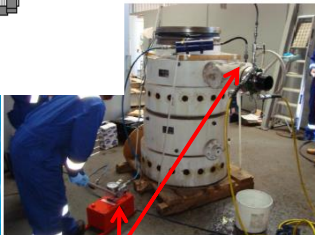
Commenced pumping Mac-Pac through "Model D" grease injection fitting on valve
