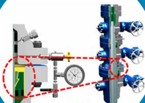
Wellhead Seal Isolation
