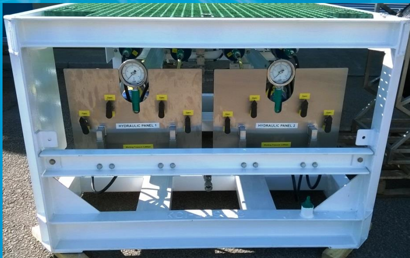
End view of Diver friendly Skid Control Panel
