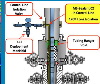
Well Abandonments
