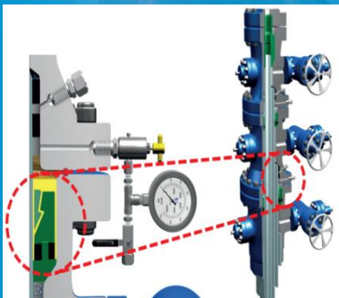
Wellhead Isolations
